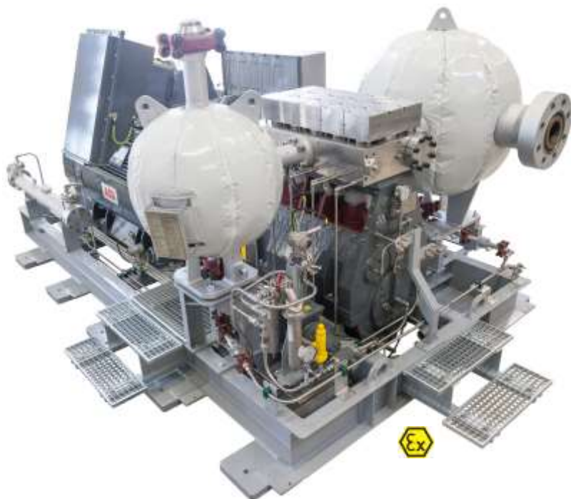
POMPE PROCESS
